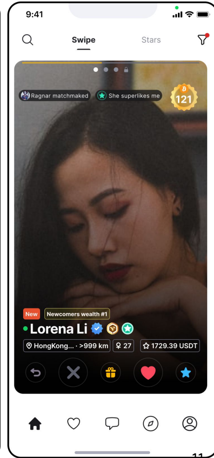
APP
