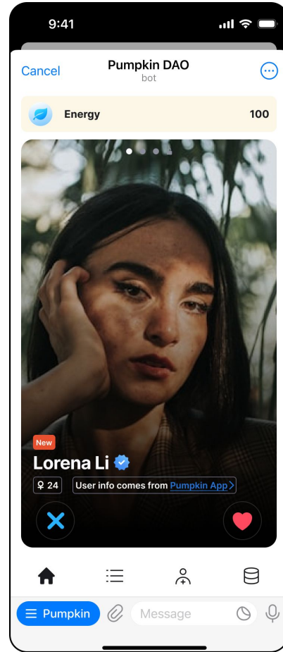
DAO
